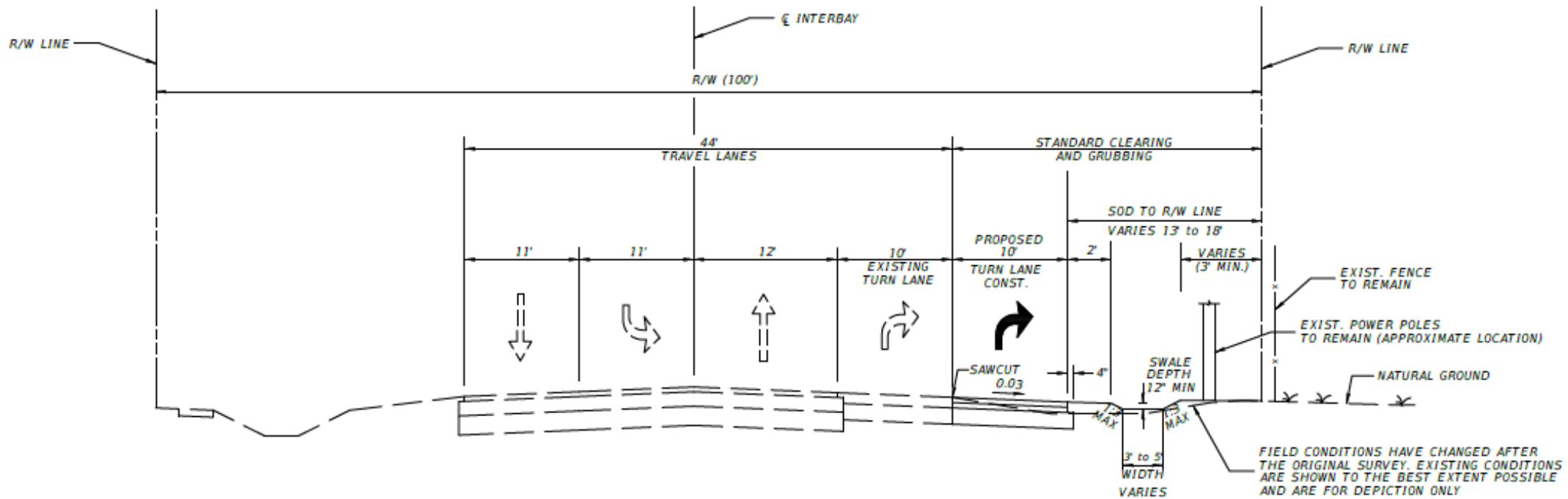
TYPICAL SECTION INTERBAY BOULEVARD STA. 14+00.00 TO STA. 19+40.00 (NTS)
