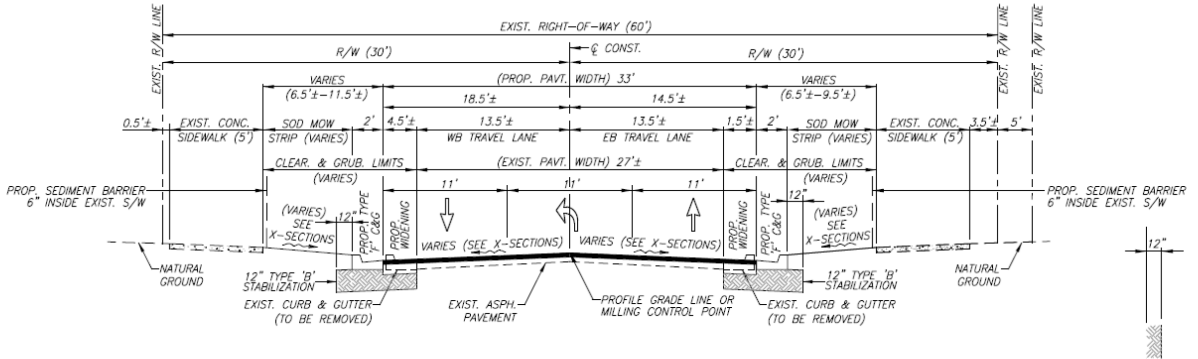
TYPICAL SECTION – INTERBAY BLVD. N.T.S.
